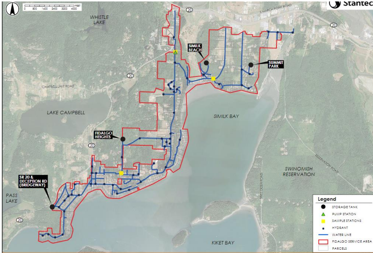
Figure 1 Water System Overview
