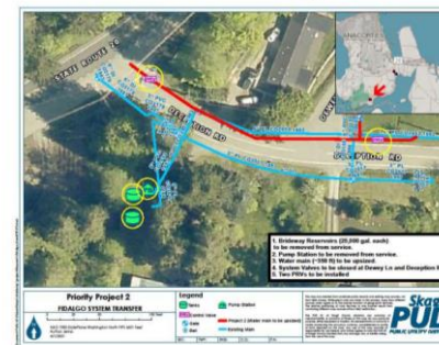
Figure 4: Bridgeway Reservoirs Abandonment, Connection to Anacortes Transmission Main and PRV Placement
