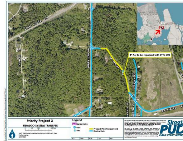
Figure 5: Satterlee, Gibraltar Rd to Mashie Street Pipeline Replacement
